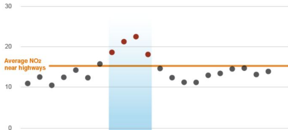
NO 2 concentrations (ppbv)
